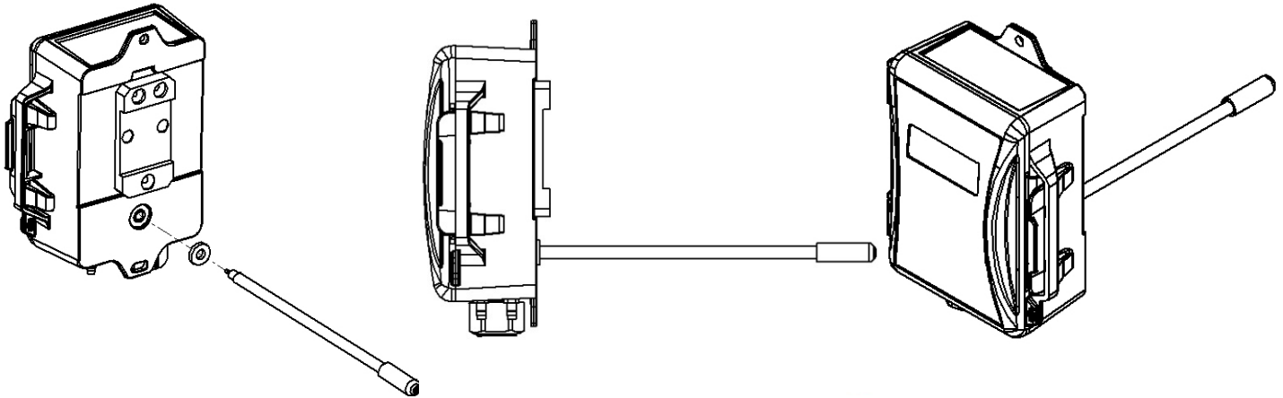
Figure 1: DPA3 Pitot Tube Installation
