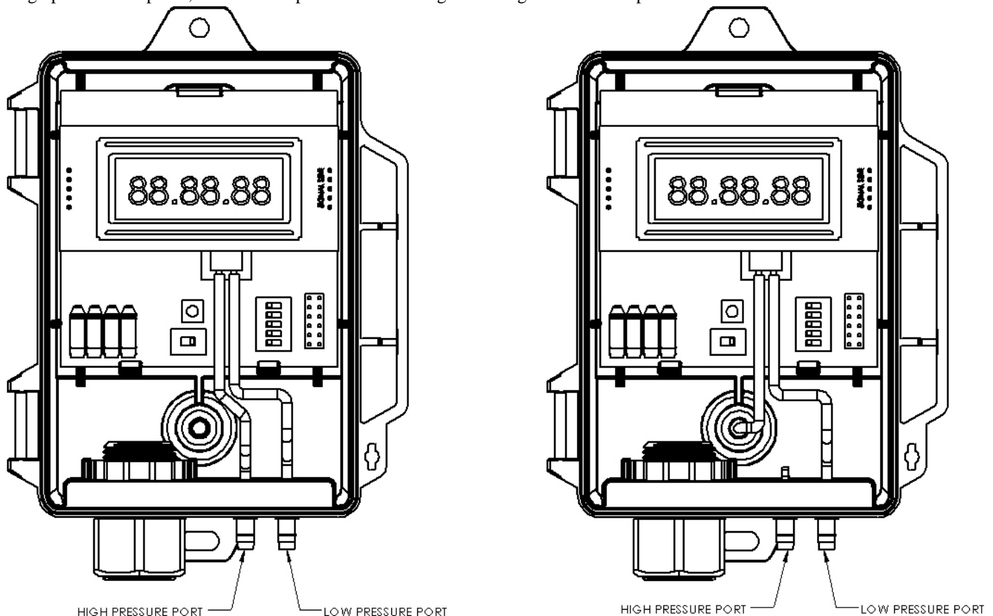
Figure 2: Pitot Tube Installation
